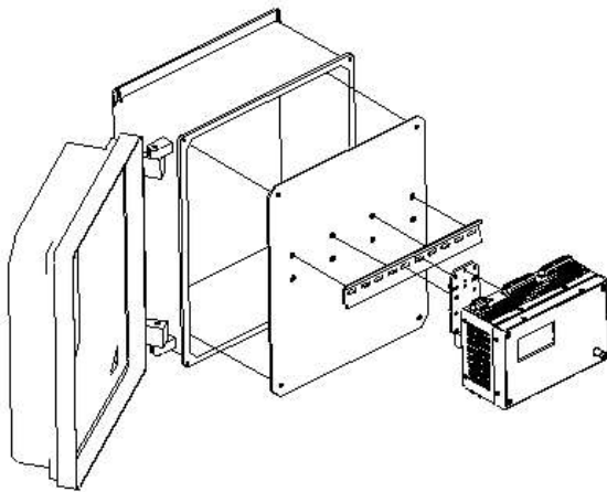
Figure 3: NEMA 4X/IP66_WP_Housing
