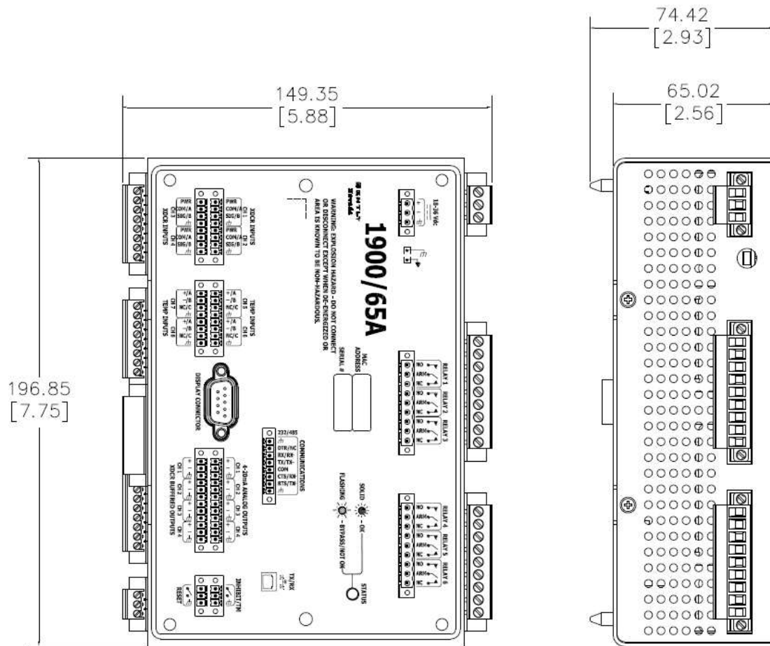
Figure 1: Monitor Module Dimensions
