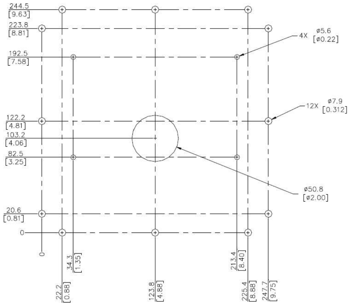
Figure 5: Weatherproof Door Drill Pattern
