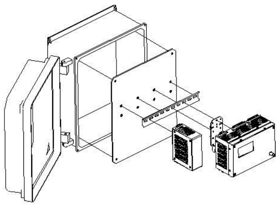
Figure 4: 1900/55 Replacement Kit
