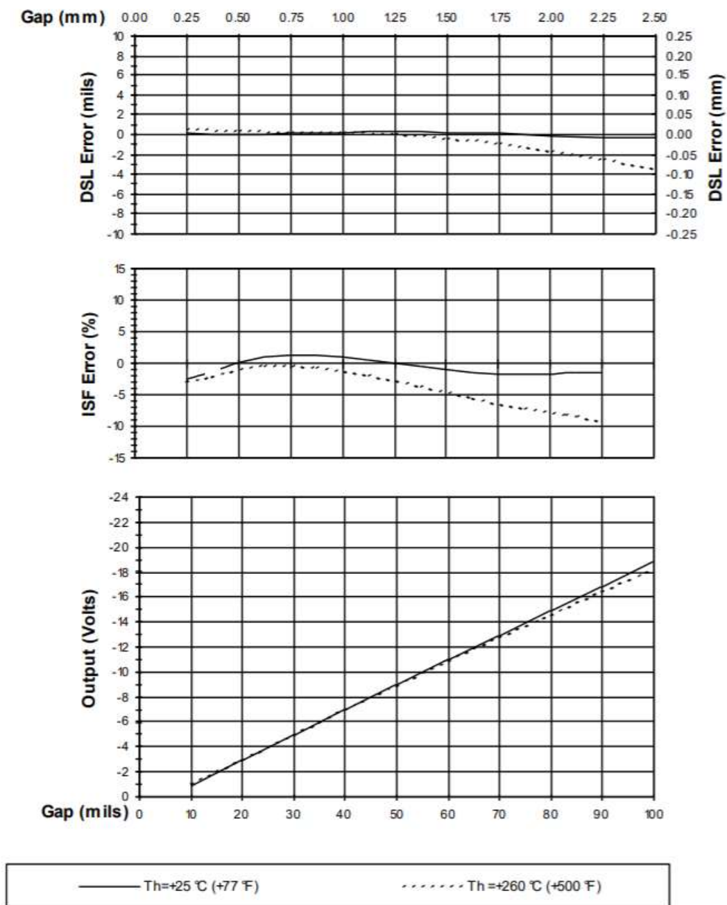
Figure 8: Typical 3300 XL Extended Temperature Range Probe and 4 m Extended Temperature Range Extension Cable at T_h (Proximitor Sensor and Probe Tip with 1-foot Cable are at +25^{\circ}\text{C} )
