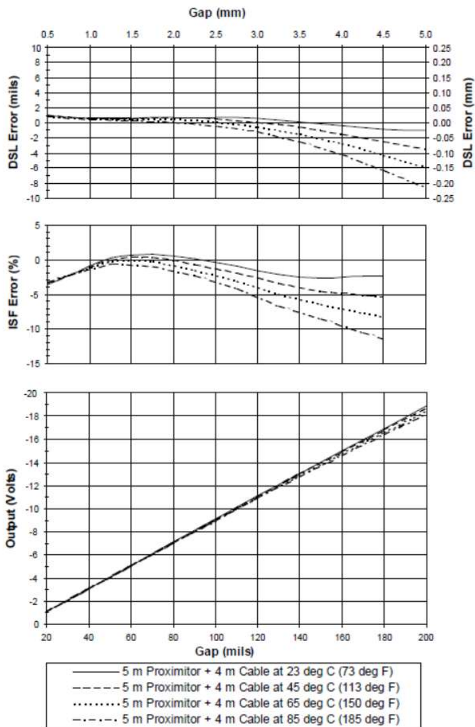
Figure 6: Typical 3300 XL 11 mm 5 m Proximity Sensor with 4 m Extension Cable @ High Temperature
