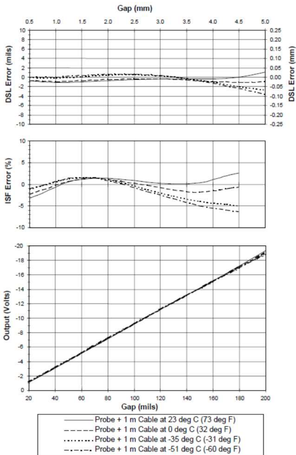
Figure 3: Typical 3300 XL 11 mm Probe + 1 m Cable @ Low Temperature (Proximator Sensor + 4m of Extension Cable @ 25 °C)
