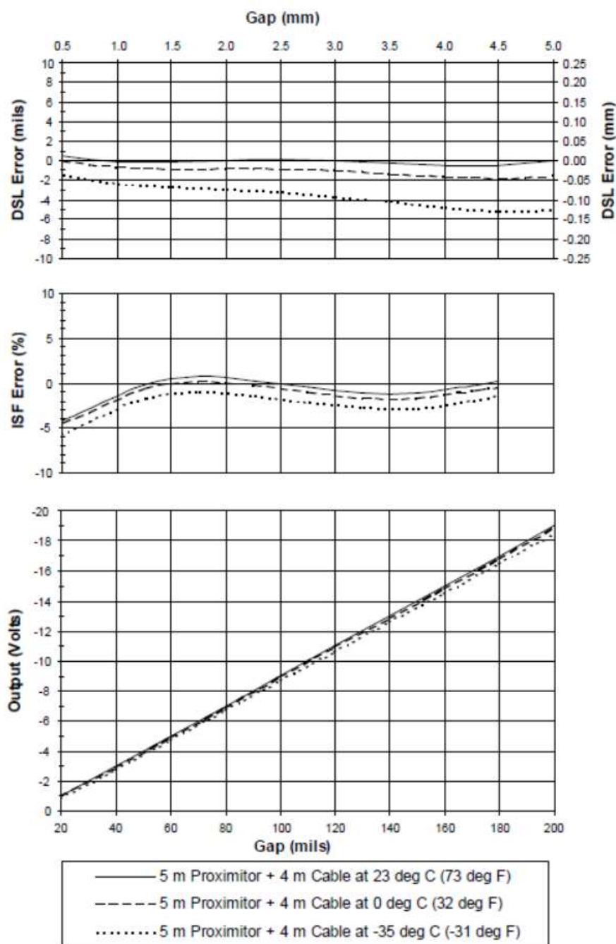
Figure 5: Typical 3300 XL 11 mm 5 m Proximity Sensor with 4 m of Extension Cable @ Cold Temperature (Probe is at 25°C)
