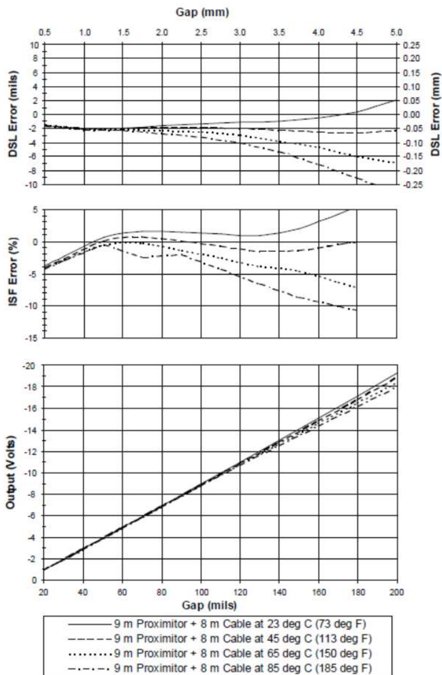
Figure 8: Typical 3300 XL 11 mm 9 m Proximity Transducer with 8 m of Extension Cable @ High Temperature (Probe is at 25°C.)
