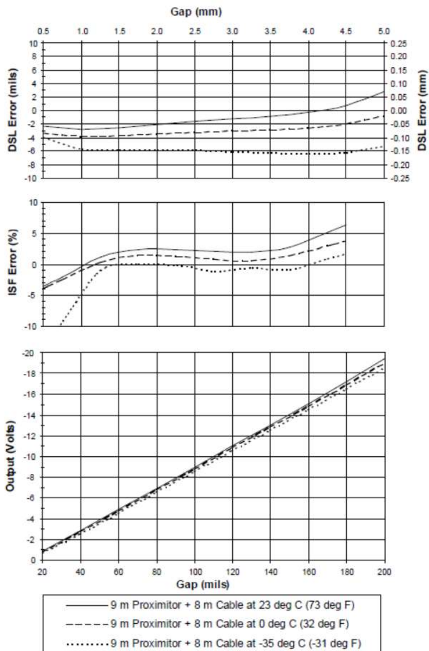
Figure 7: Typical 3300 XL 11 mm 9 m Proximator Sensor with 8 m of Extension Cable @ Low Temperature (Probe is at 25°C)
