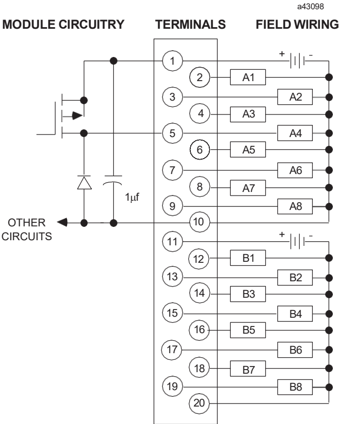
Figure 7-22. IC693MDL740 Output Module Field Wiring
