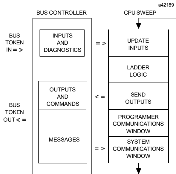
Figure 4. CPU Sweep
