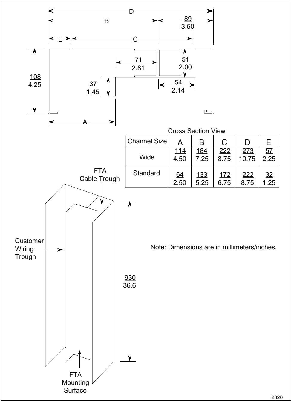
Figure 9-15 illustrates the FTA Mounting Channel dimensions. Figure 9-15 FTA Mounting Channel Dimensions
