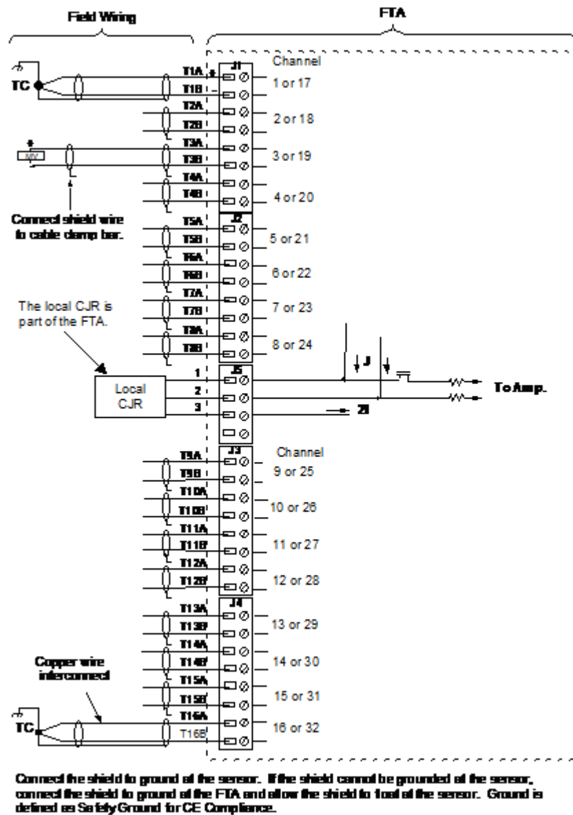
Figure 7.5 Field Wiring Connections to LLMUX2 RTD FTA
