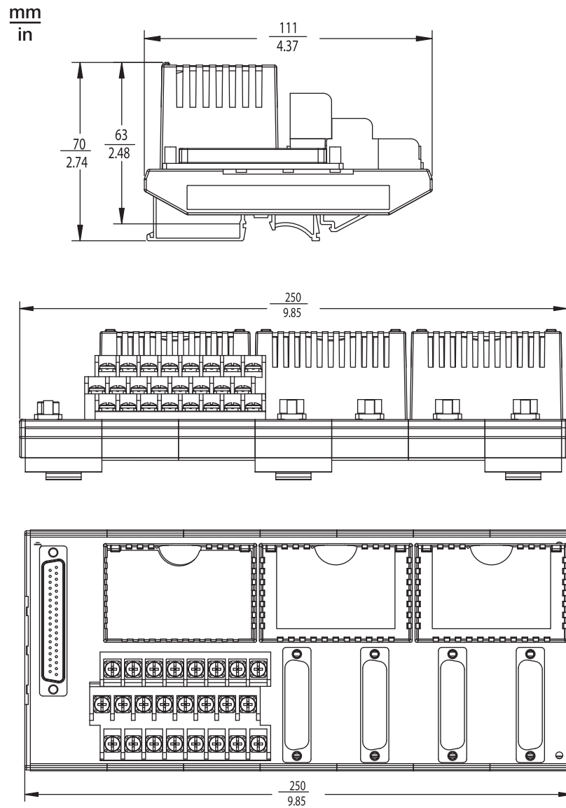
Ring Lug Termination Assembly (P0926PA) (1)
