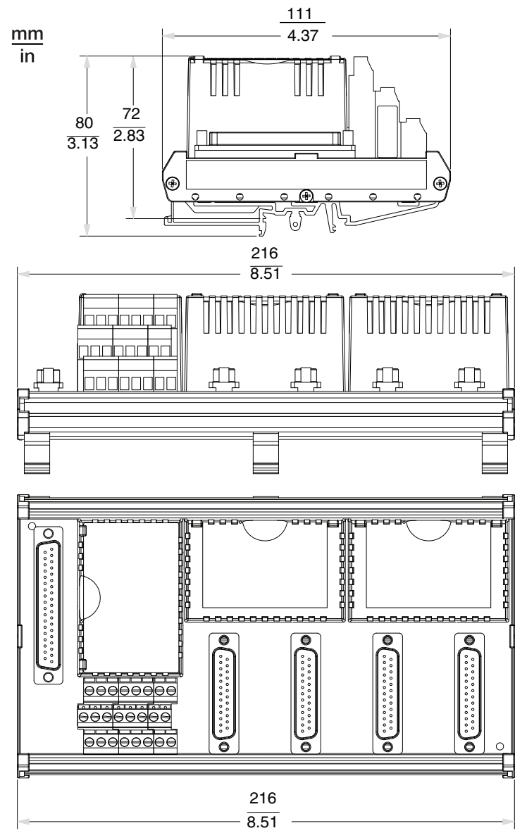
Compression Screw Termination Assembly (RH926GH (supersedes P0926GH))
