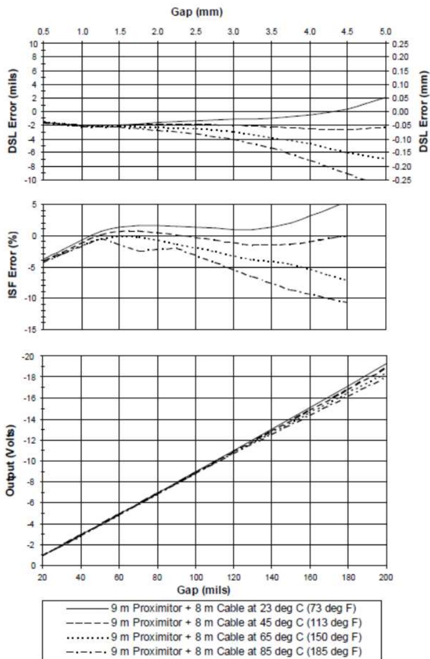
Figure 8: Typical 3300 XL 11 mm 9 m Proximity Transducer with 8 m of Extension Cable @ High Temperature (Probe is at 25°C.)
