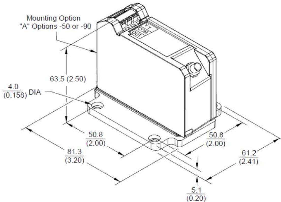
Figure 15: Panel Mount 3300 XL 11 mm Proximity Transducer
