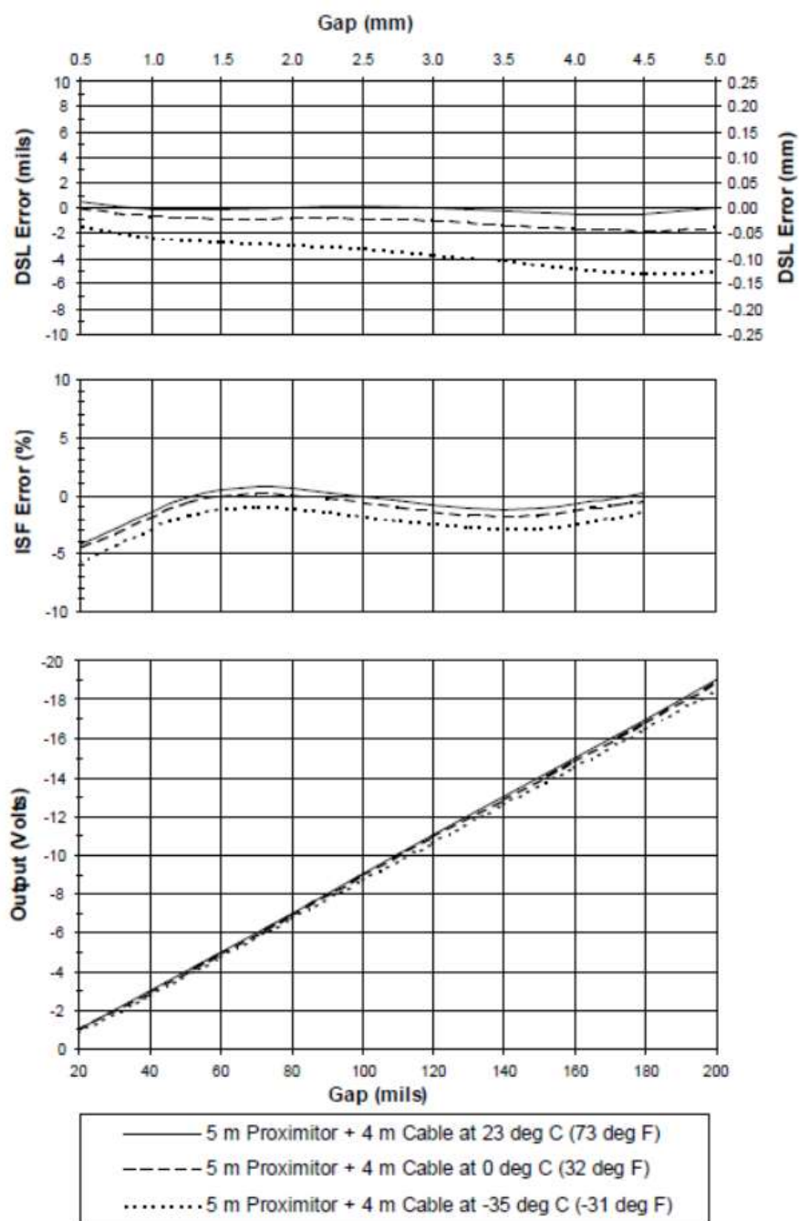
Figure 5: Typical 3300 XL 11 mm 5 m Proximity Sensor with 4 m of Extension Cable @ Cold Temperature
