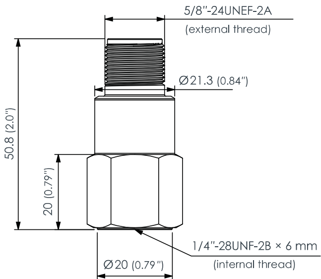
CE687 accelerometer
