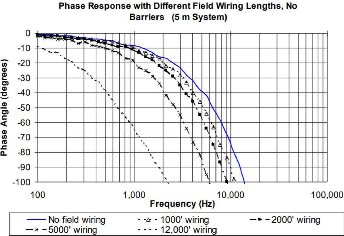
Figure 11: Phase Response, Typical 3300 XL 8 mm 5 m or 1 m System with Varying Lengths of Field Wiring Attached, No Barriers
