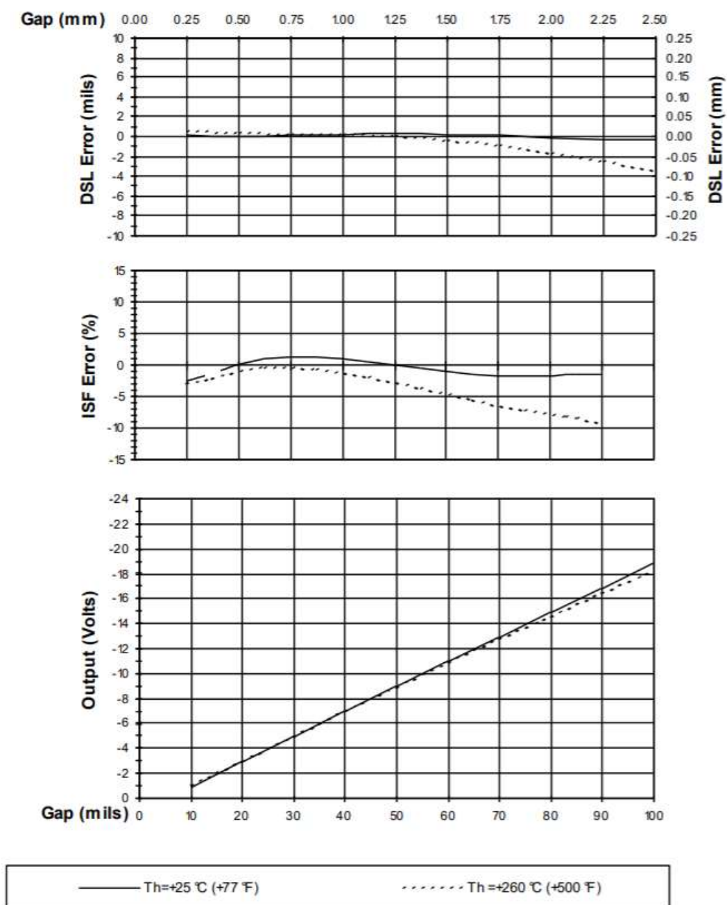
Figure 8: Typical 3300 XL Extended Temperature Range Probe and 4 m Extended Temperature Range Extension Cable at T_h (Proximitor Sensor and Probe Tip with 1-foot Cable are at +25\text{ }^{\circ}\text{C} )
