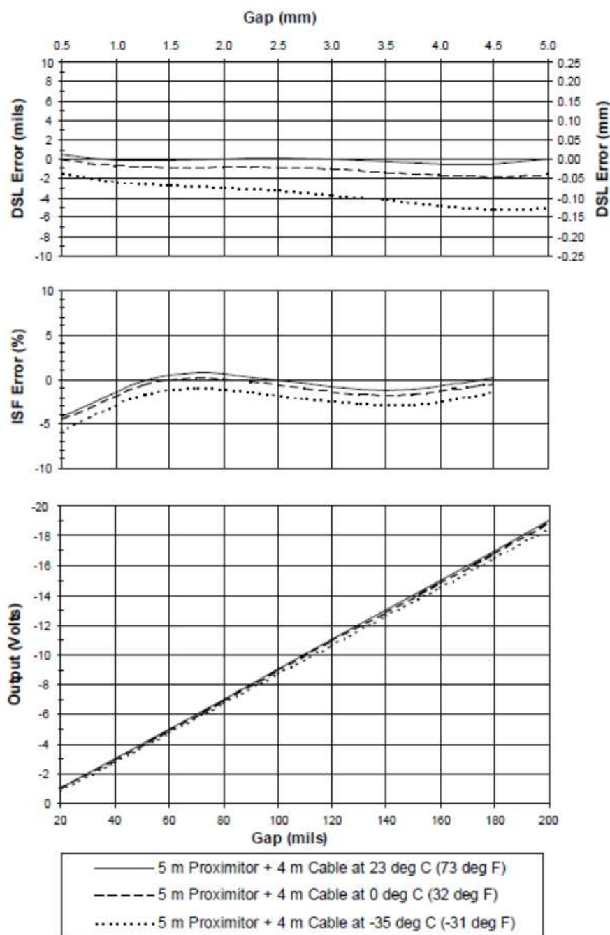
Figure 5: Typical 3300 XL 11 mm 5 m Proximity Sensor with 4 m of Extension Cable @ Cold Temperature
